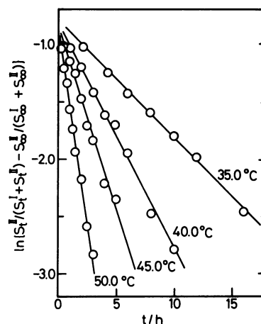
Fig. 4. The plots of \ln[S_t^{\text{II}}/(S_t^{\text{I}}+S_t^{\text{II}}) - S_\infty^{\text{II}}/(S_\infty^{\text{I}}+S_\infty^{\text{II}})] against time for the epimerization of \Delta(R)\Lambda(S) -[Co(dbme) 2 (CH 3 SeCH 2 CH 2 NH 2 )] + at 35.0, 40.0, 45.0, and 50.0 °C ( S_t^{\text{I}} , S_t^{\text{II}} , S_\infty^{\text{I}} , and S_\infty^{\text{II}} denote the areas of bands I and II at time t and at infinite time).
